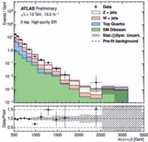
Figure 2: Transverse mass distribution of the \nu\nu J system in the high purity signal region. The pre-fit background (red-dashed line) slightly differs from the background stack compared with data in the bottom panel.
