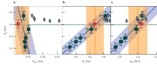
Figure 3: Correlation between the neutron skin, r.m.s. point-neutron radius and electric dipole polarizability of ^{48}\text{Ca} versus the r.m.s. point-proton radius. [From (Hagen et al. 2016)]
