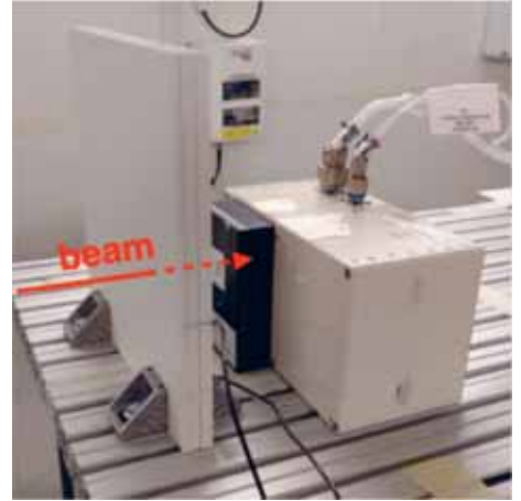
Figure 1: Single SDU test configuration: the first element in line is the plastic degrader (2.5 cm thick), followed by the scintillation counter (black box) and the SDU.
