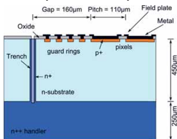
Figure 1: Active edge sensor cross section.
