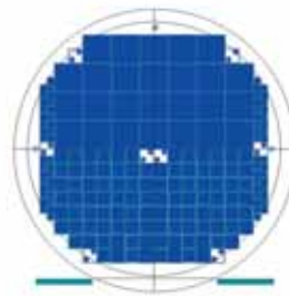
Figure 2: Wafer layout drawing.
