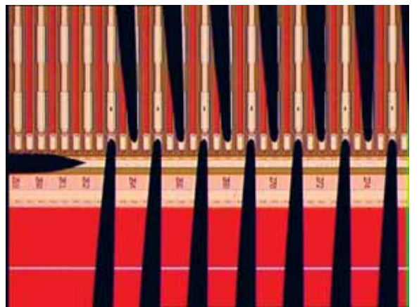
Figure 2: Test DC pad.
