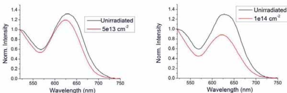
Figure 1: Photoluminescence spectra of unirradiated and irradiated samples ( 5 \times 10^{13} and 10^{14} ions/cm 2 ). The spectra were collected with the excitation wavelength of 470 nm.
