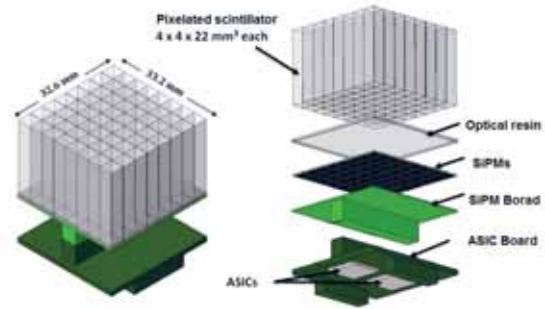
Figure 9: A 8 \times 8 pixels GDM schematic representation. Two 32-channels ASICs are in use in order to manage the 64 signals incoming from the SiPMs.
