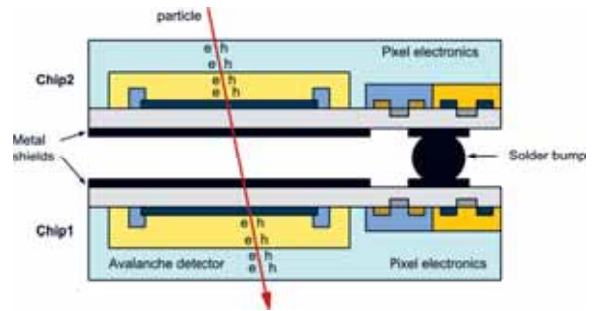
Figure 1: Concept view of a two-tier avalanche pixel
