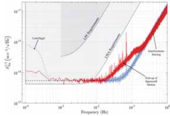
Figure 3: Spectrum of differential acceleration noise measured by LISA Pathfinder shown together with the LISA Pathfinder and the LISA requirement (Armano et al. 2016b).
