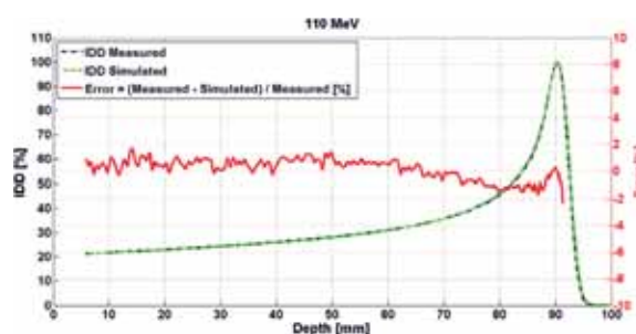
Figure 6: Comparison between measured and simulated integral depth dose after ‘tuning’ the energy spectrum for 110 MeV (see (Fracchiolla et al. 2015)).
