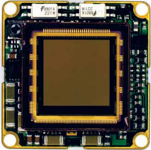
Figure 3: MQ042MG-CM-BRD Ximea sensor, in use at TIFPA as building block of a particle tracker. 5.5\text{ }\mu\text{m} pixel size, 10 bit ADC, 90 fps acquisition rate.
