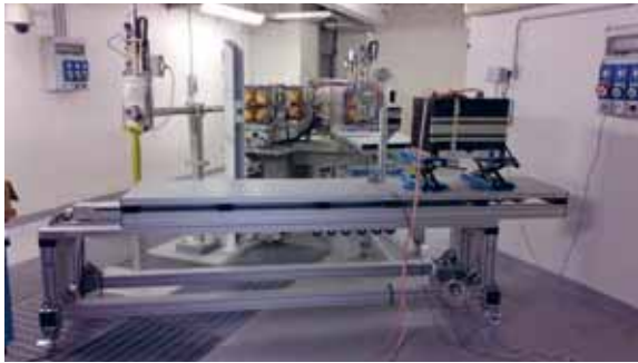
Figure 3: The experimental hall at the APSS proton-therapy center with the two positioning tables. The 275 cm \times 60 cm table is visible in foreground. The 100 cm \times 60 cm table is in the background, below the terminal point of the 30° beamline. The 0° beamline is also clearly visible on the left hand side of the picture.
