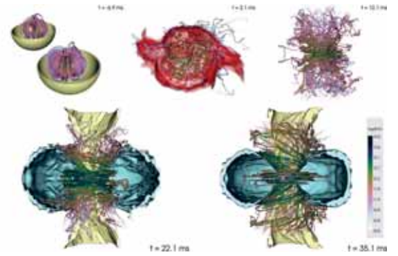
Figure 1: Simulation of a binary neutron star merger. The different panels show different stages of the evolution highlighting in particular the magnetic field structure. The last two panels show the final stages of the simulation where a black hole surrounded by an accretion disk is formed. In this case a magnetized low density funnel is also formed, which could launch a relativistic jet and possibly produce a short gamma-ray burst at a later time. The color of the field lines gives a rough indication of the field strength. Source: (Kawamura et al. 2016).
