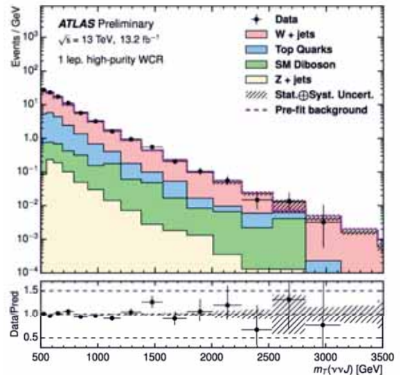
Figure 1: Transverse mass distribution for the W high purity control region. Most events come from W + jets processes (pink), as expected. The bottom panel shows the ratio of the observed data to the predicted background.
